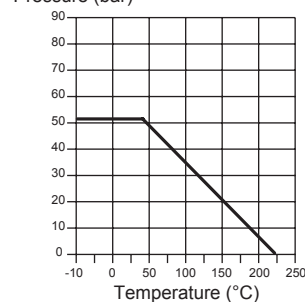
KH 2T F-KFM, ½"-4", 300 lbs. Pressure (bar)
