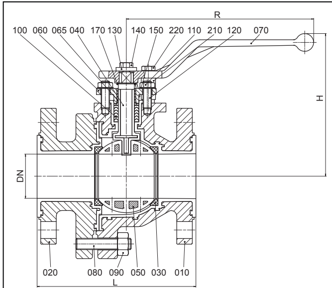
Flange Connections
