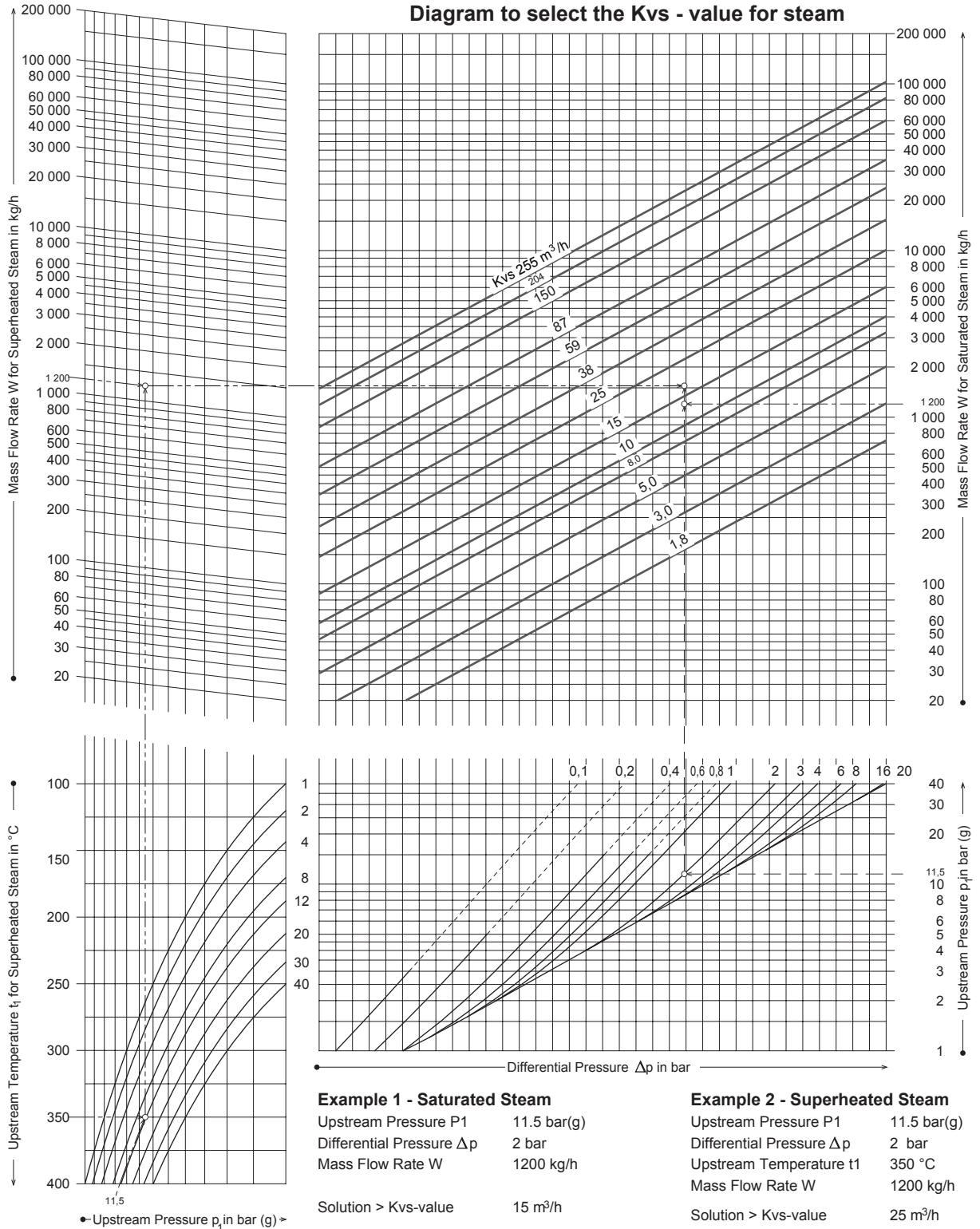
Kvs Values for Selection of Valve Size
